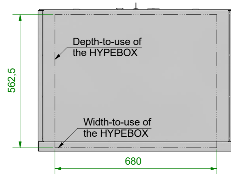
Top View 1 : 10
