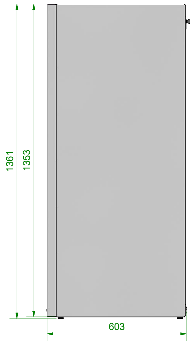
Righthand View 1 : 10
